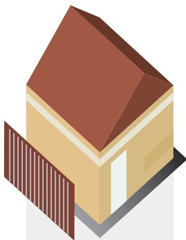
Scheme 10
