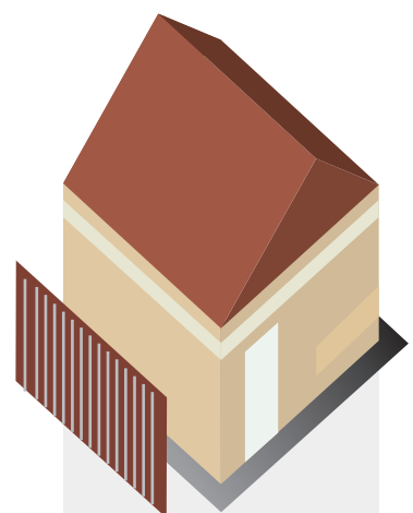
Scheme 15
