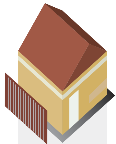
Scheme 12
